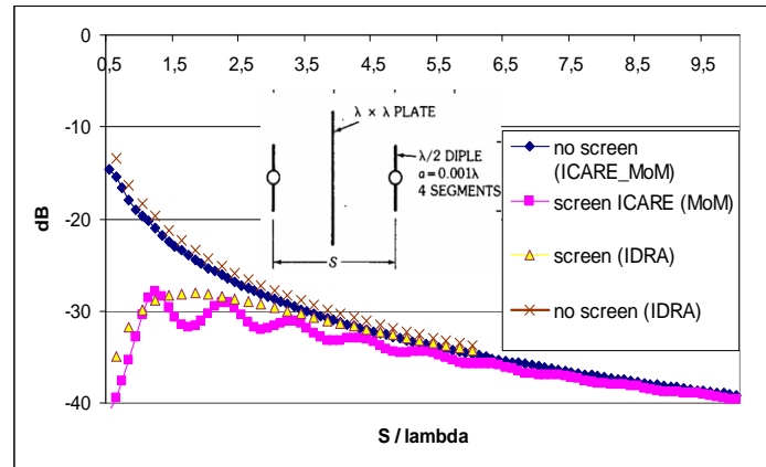
Figure 9 : Coupling between two dipole antennas separated by a square plate
