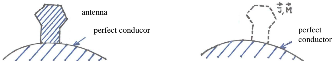
Figure 5 : Equivalence theorem for the hybridization of an integral equation method with asymptotic solutions
